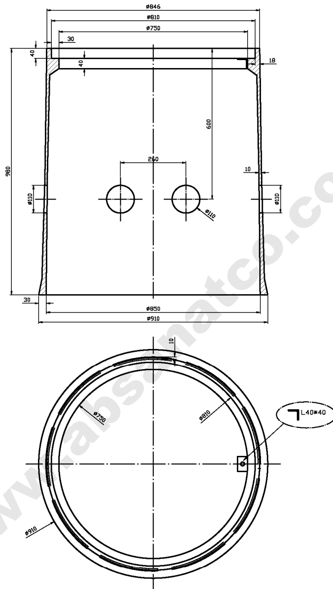
HANDHOLE SIDE VIEW
