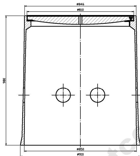
ASSEMBLY FRONT VIEW
