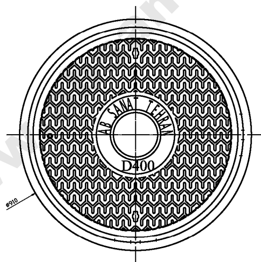
ASSEMBLY TOP VIEW
