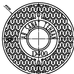
COVER TOP VIEW
