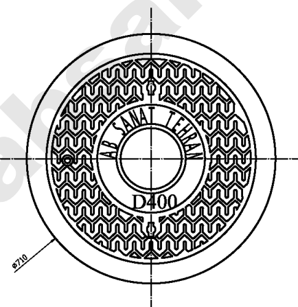
ASSEMBLY TOP VIEW
