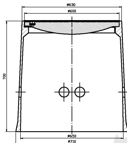
ASSEMBLY FRONT VIEW
