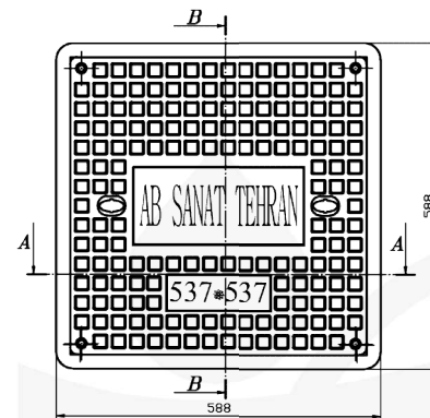
ASSEMBLY TOP VIEW
